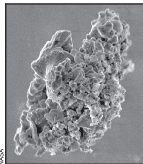
This tiny speck of dust shed from a comet is only about 6 by 10 micrometers, but it is huge compared to interstellar dust. Most interstellar dust grains are one micrometer (the size of the small white scale bar) or smaller.
